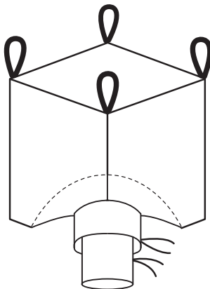
open mouth/ discharge valve
